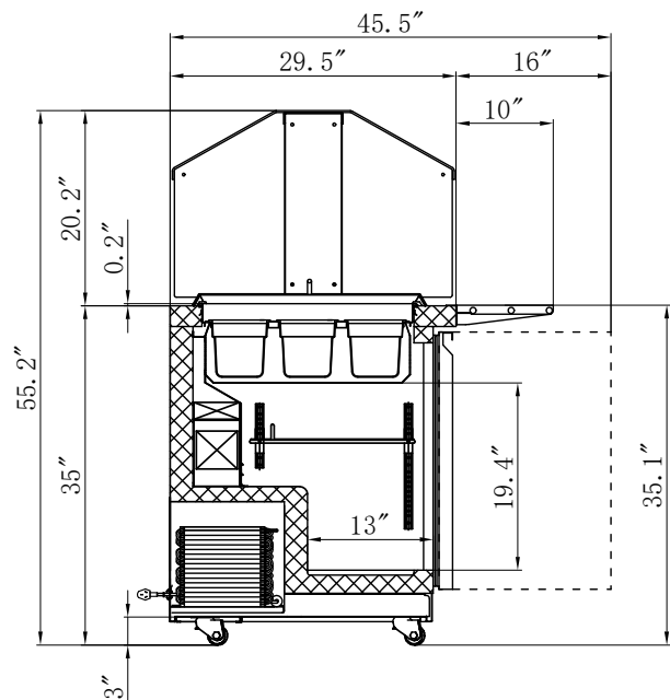
SECTION VIEW
