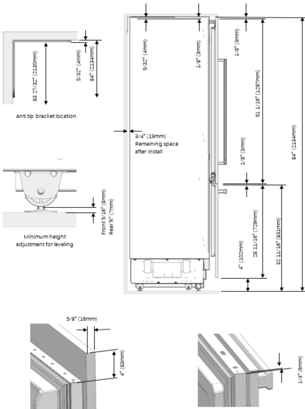
Assembly dimension between Wood panel and fridge door
