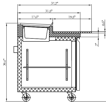
SECTION VIEW
