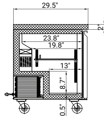
SECTION VIEW
