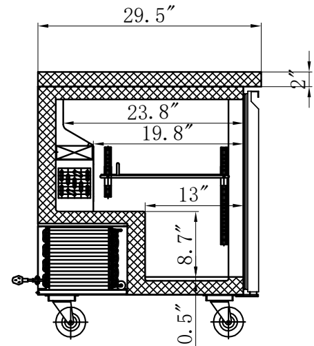
SECTION VIEW
