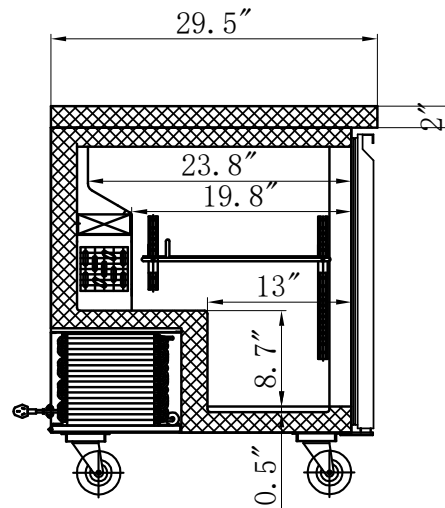
SECTION VIEW
